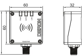
KTSR-A-H-MR-P6032
