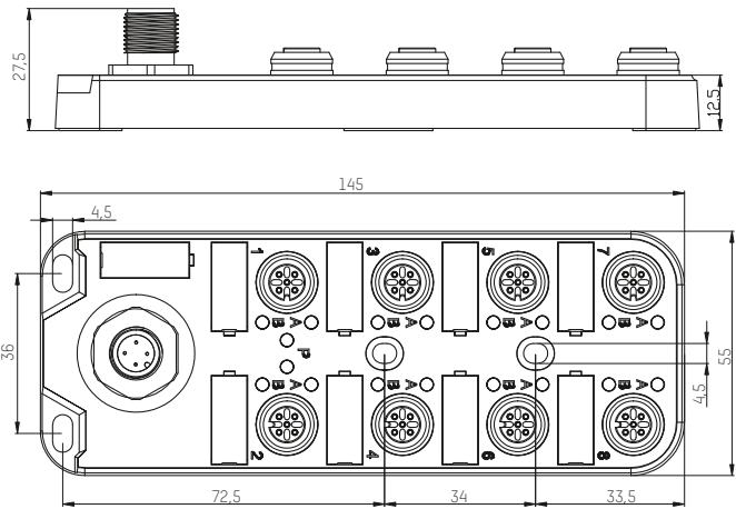
KTSN-S-P-IO-08DP-M12/EXT1 KTSN-S-P-IO-08DN-M12/EXT1
