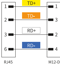
M12 D-CODE
